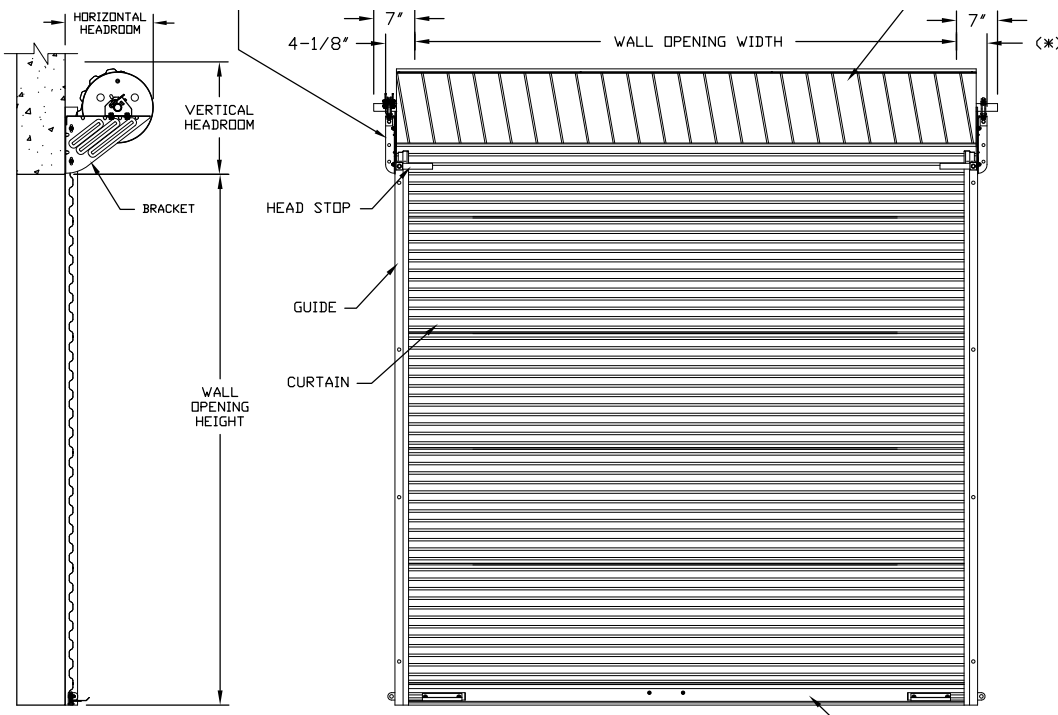
HEADROOM REQUIRED
